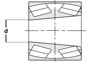
Tapered Bore (K30) (1:30)
