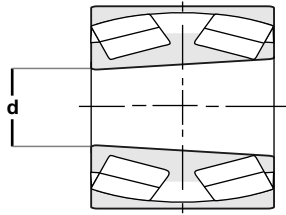
Tapered Bore (K) (1:12)
